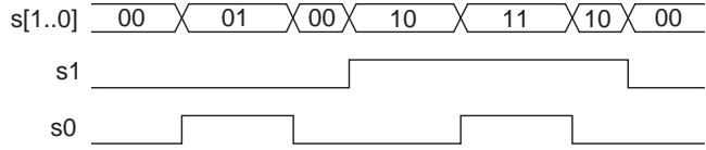
Figure 10. Waveforms Caused by Misaligned Sensors
